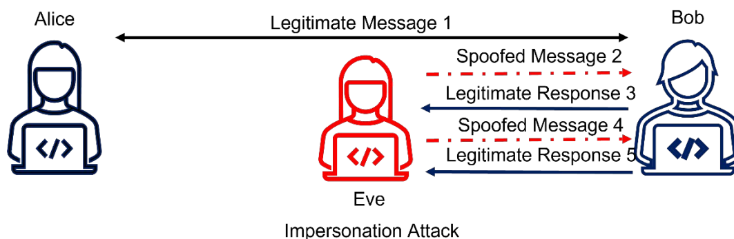
Figure 4. Impersonation Attack
