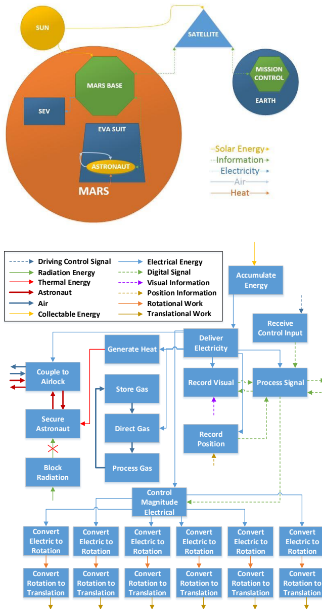
Figure 1. Simplified functional diagram of the system focusing on the astronaut (top). Simplified functional model of the Surface Exploration Vehicle (bottom).
