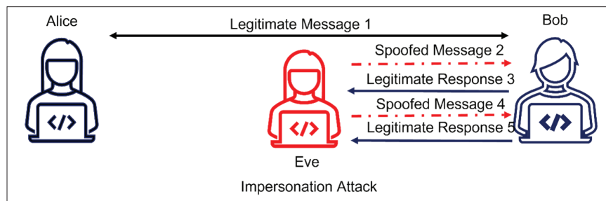
FIGURE 4. Impersonation Attack
