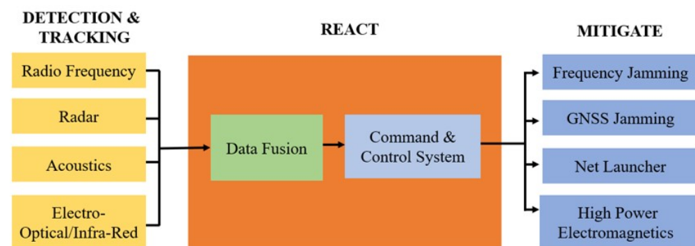
Figure 2. C-UAS network [44].
